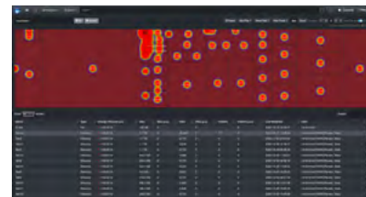
Heat Map
