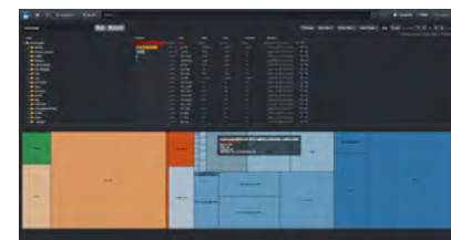
Tree Map
